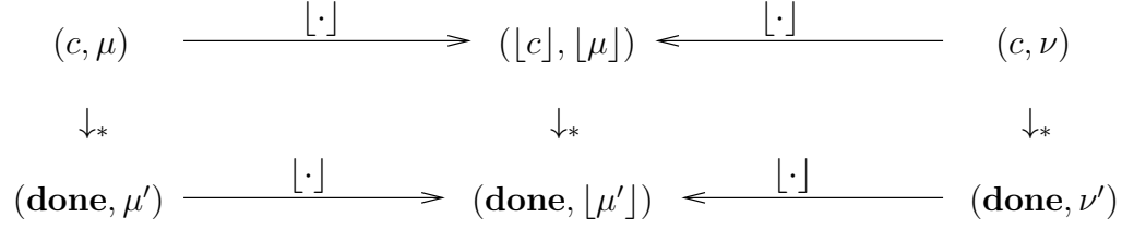
Figure 3.6: Noninterference of terminating executions
